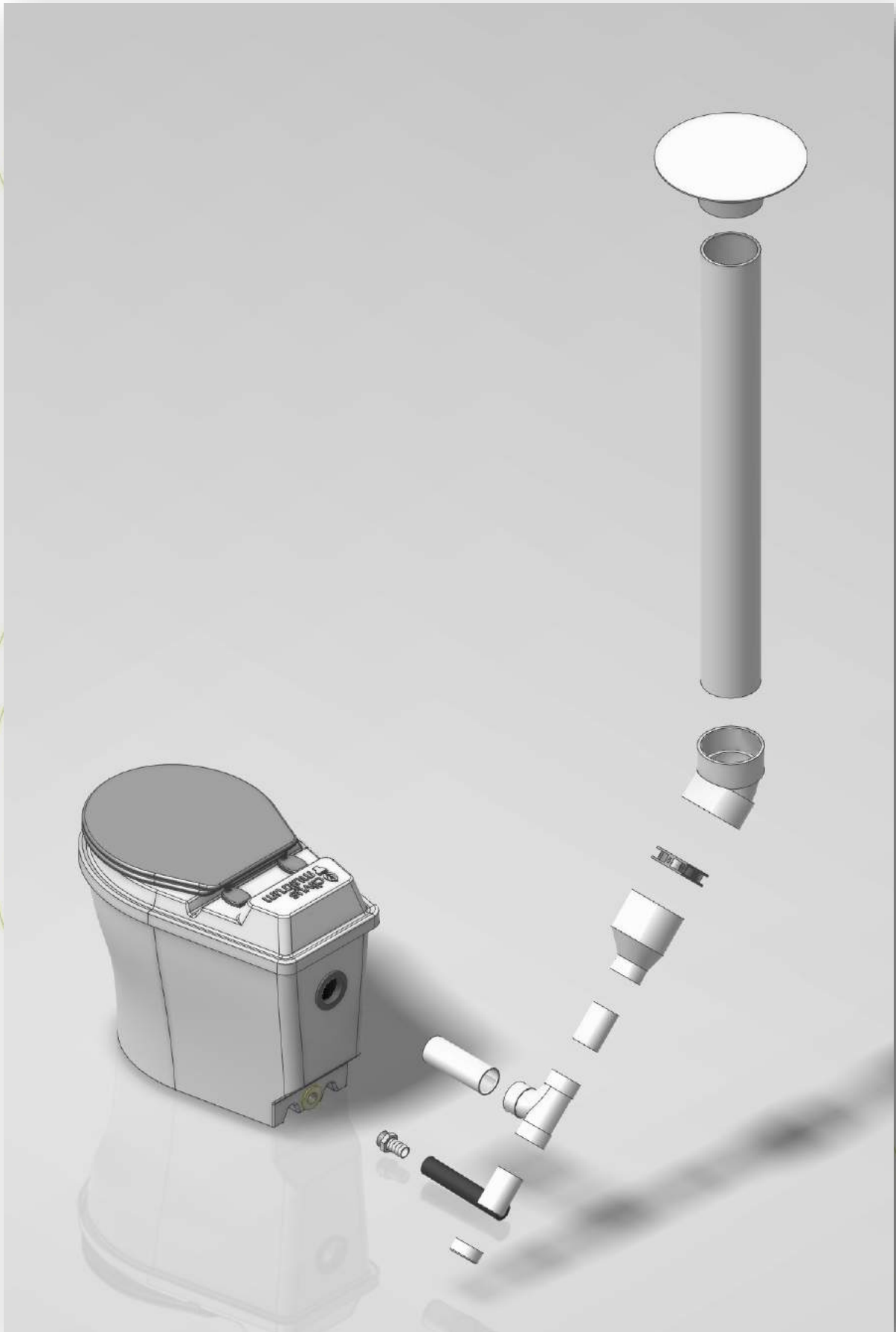
Figure 3: Ventilation pipe components break-out view
