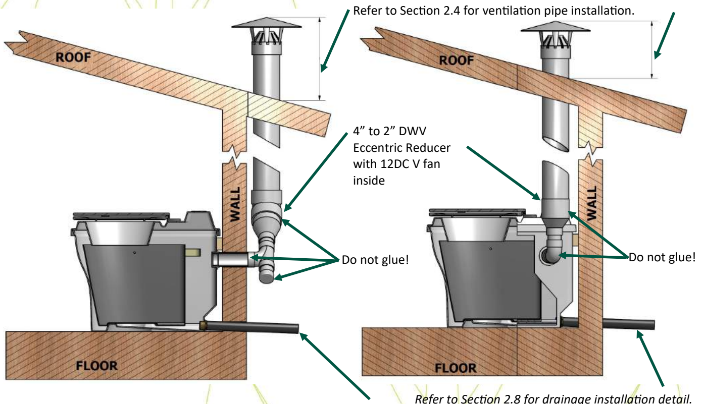
Figure 1: Ventilation pipe installed Outside.
