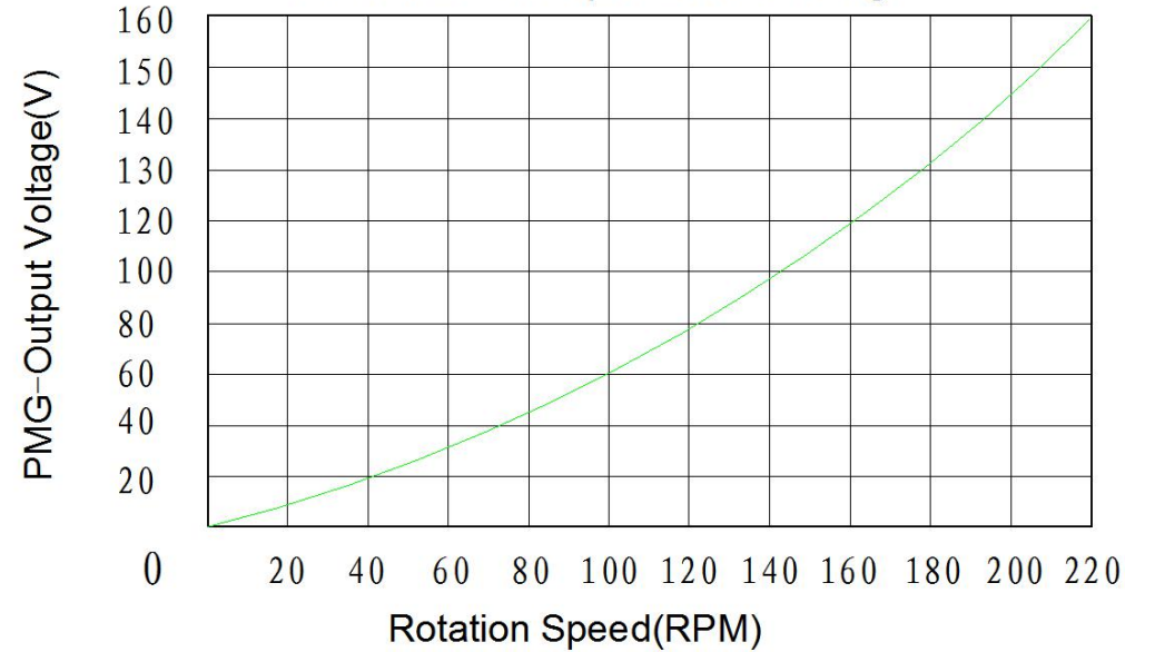
BF-PMG-2KW Open Circuit Voltage
